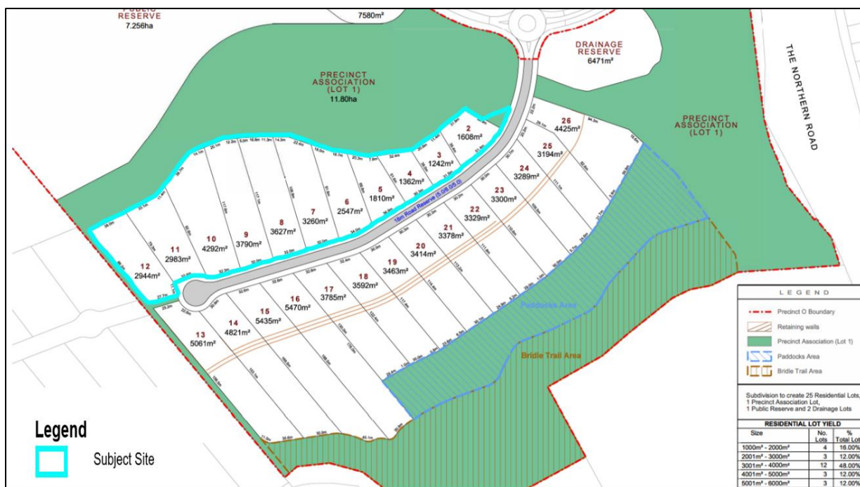
Figure 2: Subdivision Plan
